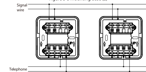
Figure 3-3 Mounting base (2)
