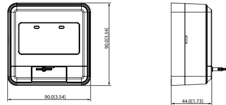
Figure 1-1 Dimensions (mm[inch])
