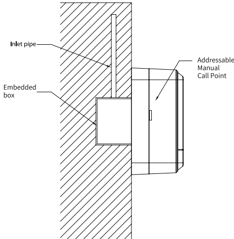
Figure 3-6 Installation (3)
