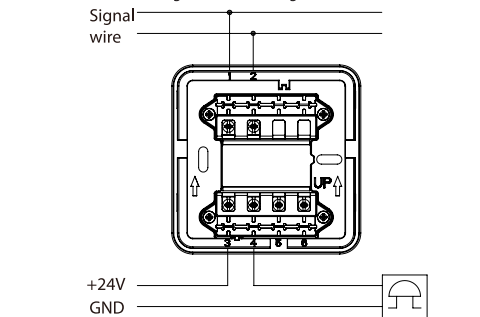
Figure 3-3 Mounting base (2)
