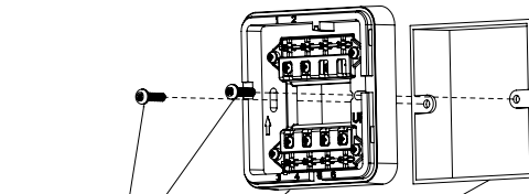
Figure 3-1 Installation (1)
