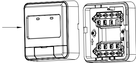
Figure 3-6 Installation (3)
