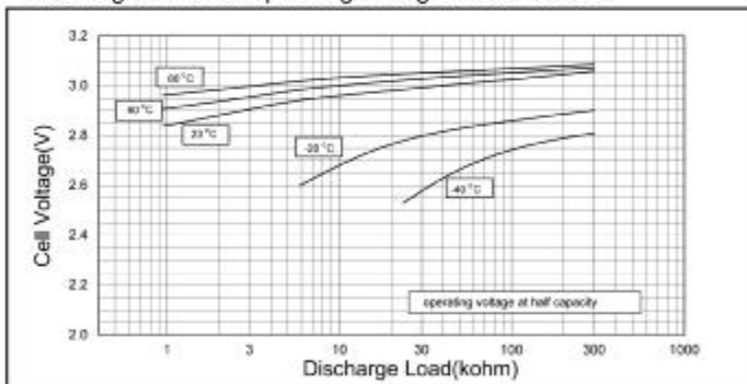
Discharge Load vs. Operating Voltage of CR12600SE
