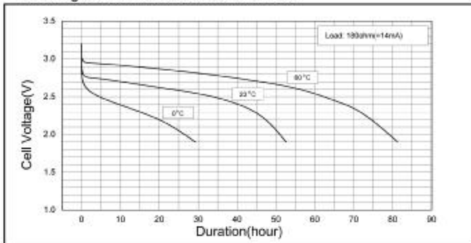
Discharge Characteristics of CR12600SE
