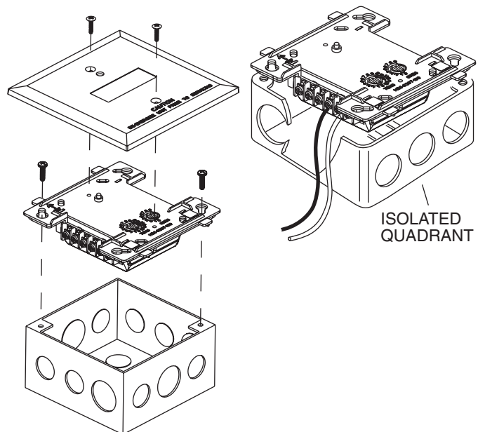
FIGURE 2. MODULE MOUNTING:
